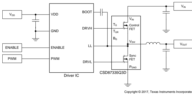
Typical Circuit
