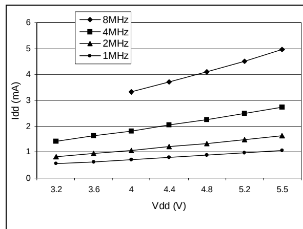
Figure 81. Typical I_{DD} in WAIT vs. f_{CPU}
