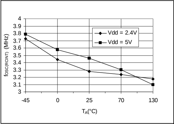
Figure 87. Typical f_{OSC(RCINT)} vs T_A
