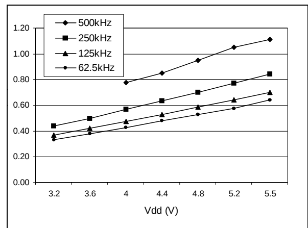
Figure 82. Typical I_{DD} in SLOW-WAIT vs. f_{CPU}
