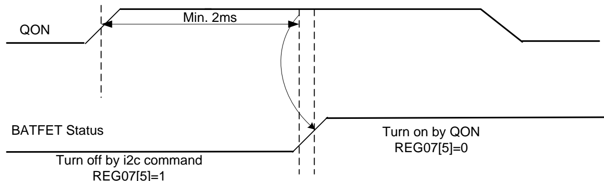
Figure 22. QON Timing
