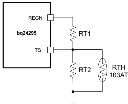
Figure 28. TS Resistor Network
