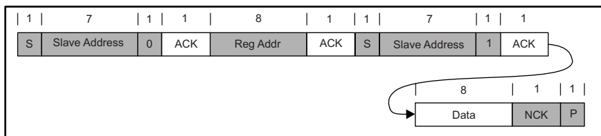
Figure 37. Single Read
