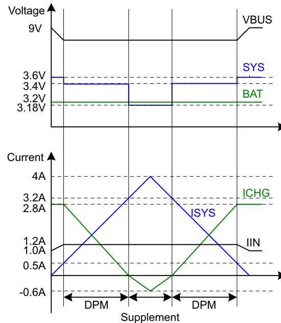
Figure 17. DPM Response
