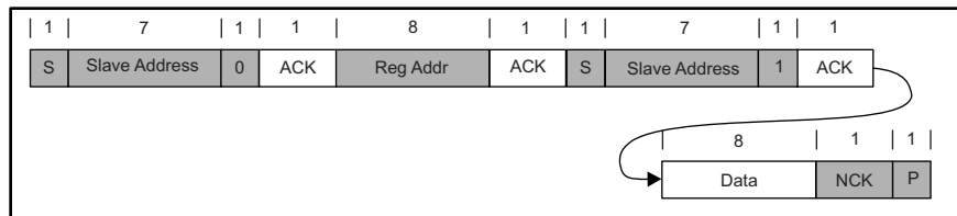
Figure 28. Single Read
