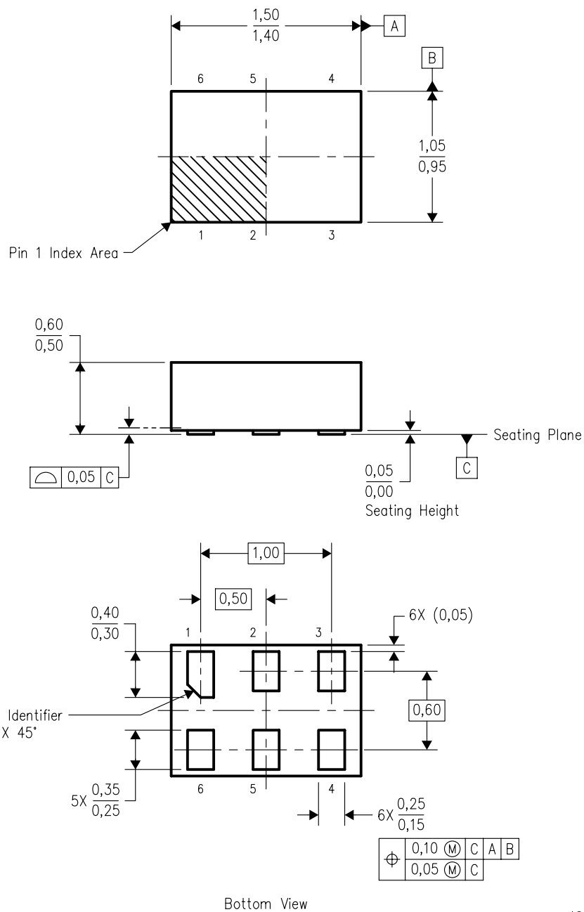
Bottom View
