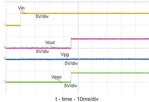
Figure 2. Power up Timing – No Battery or Load, bq24041
