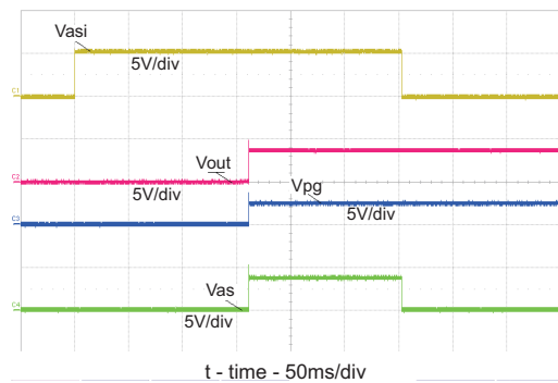
Figure 4. ASI and delayed OUT Power-up Timing – No Input, bq24041
