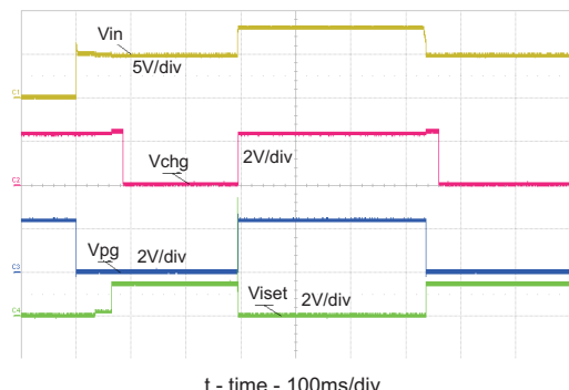
Figure 6. OVP from Normal Power-up Operation – V_{IN} 0V \rightarrow 5V \rightarrow 8V \rightarrow 5V
