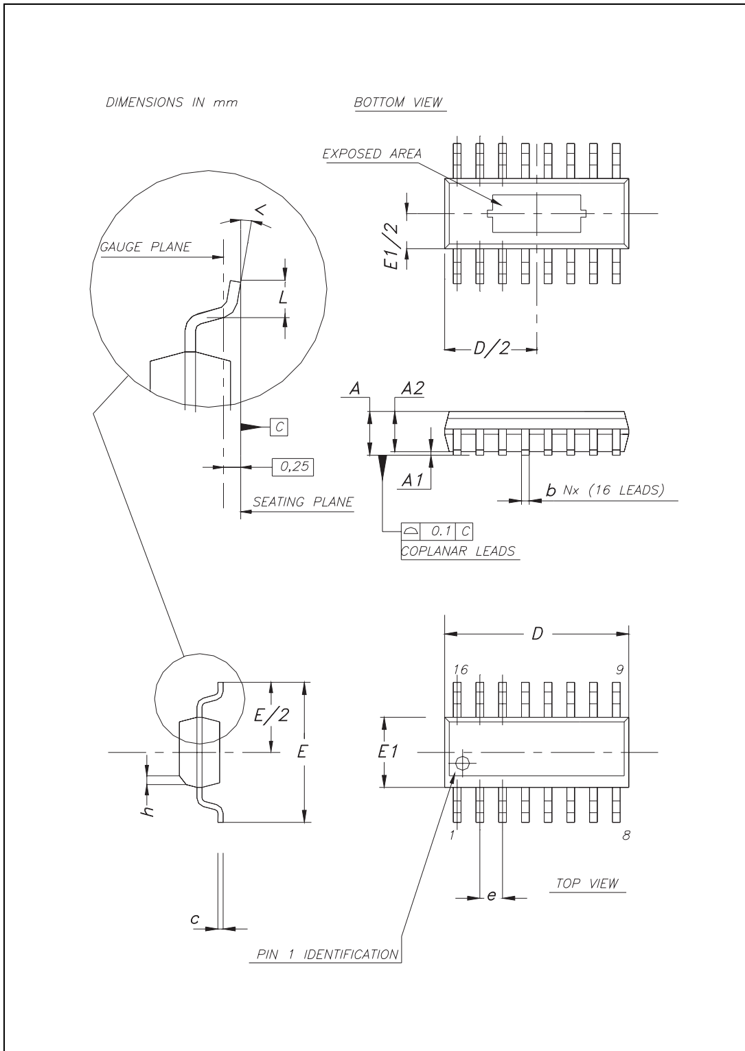
Figure 34. Package dimensions
