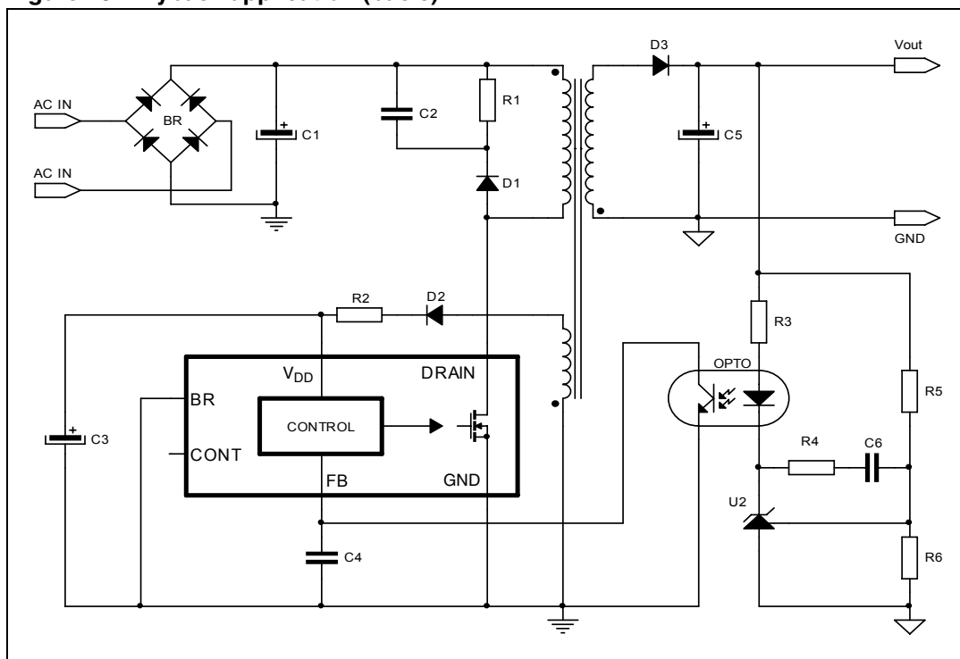
Figure 21. Flyback application
