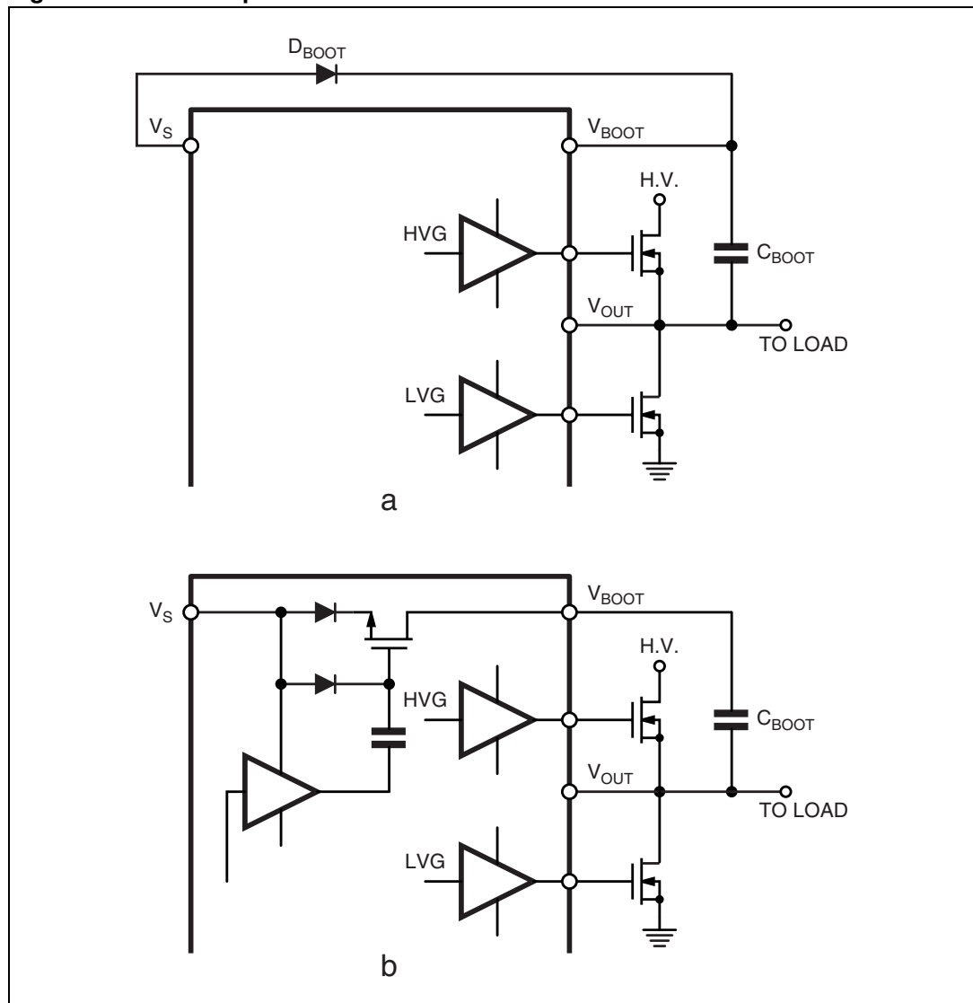
Figure 5. Bootstrap driver
