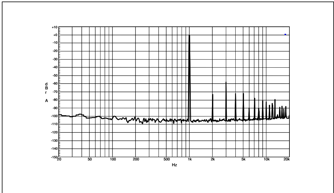
Figure 6. FFT 0 dBfs 1 kHz, Vcc = 12 V, RL = 8 Ω
