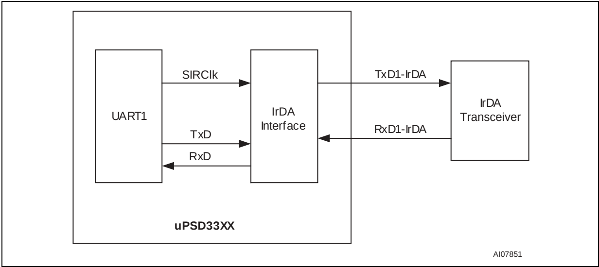
Figure 36. IrDA Interface
