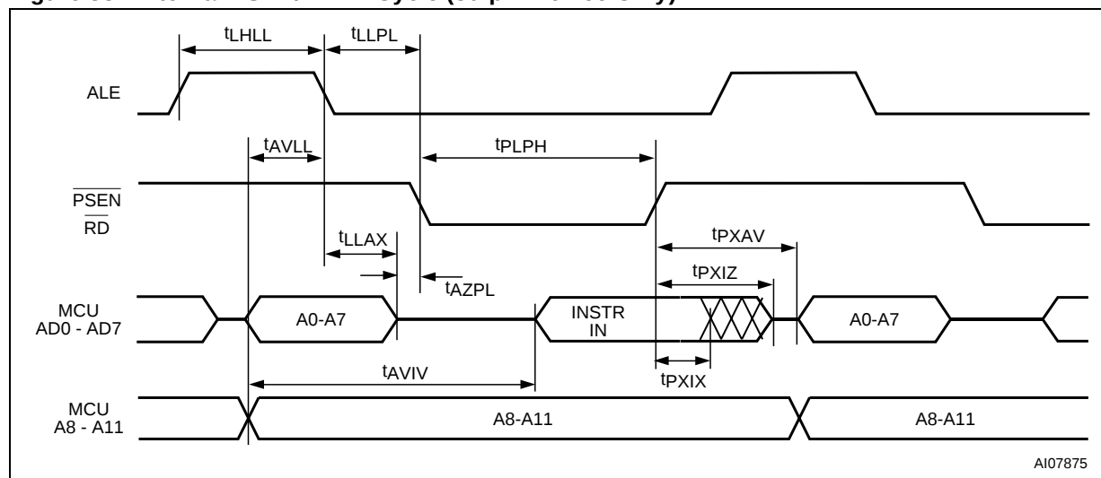
Figure 88. External \overline{\text{PSEN}} /READ Cycle (80-pin Device Only)
