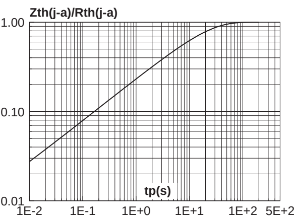
Fig 6: Relative variation of thermal impedance junction to ambient versus pulse duration.
