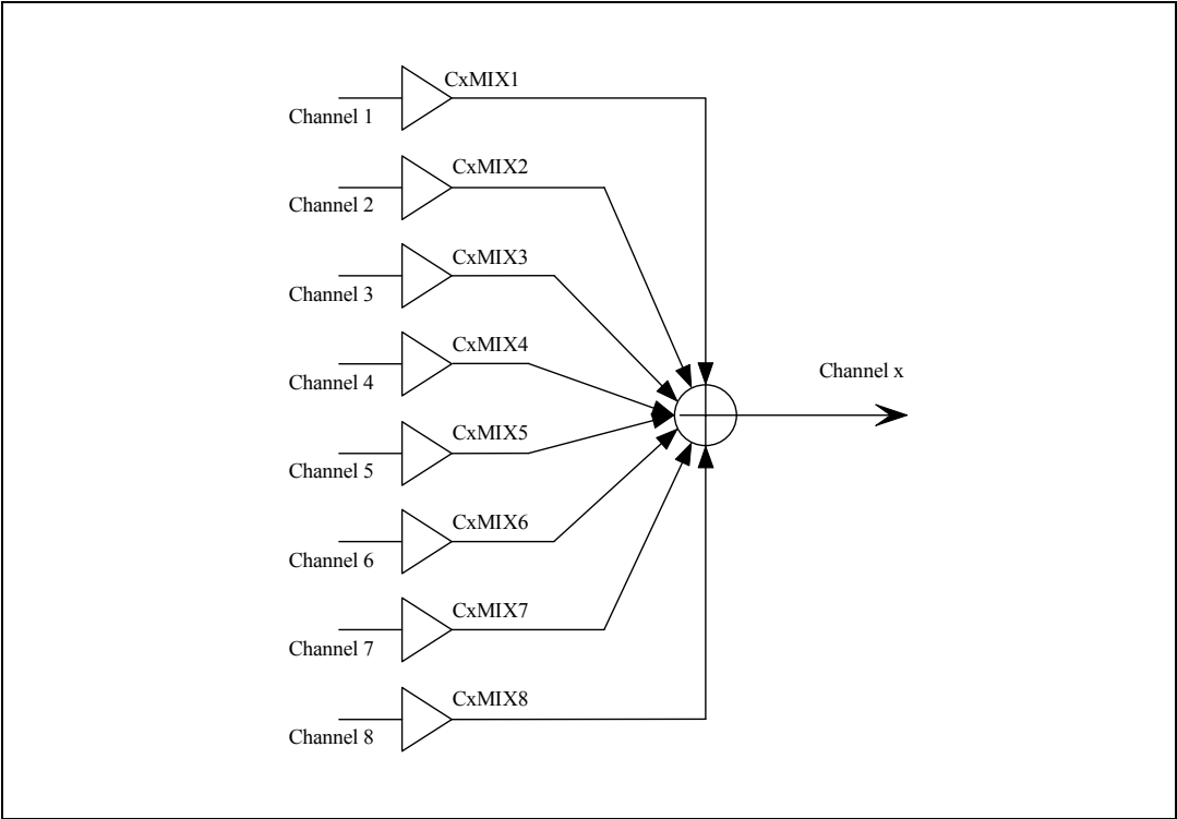
Figure 8. Channel mixer
