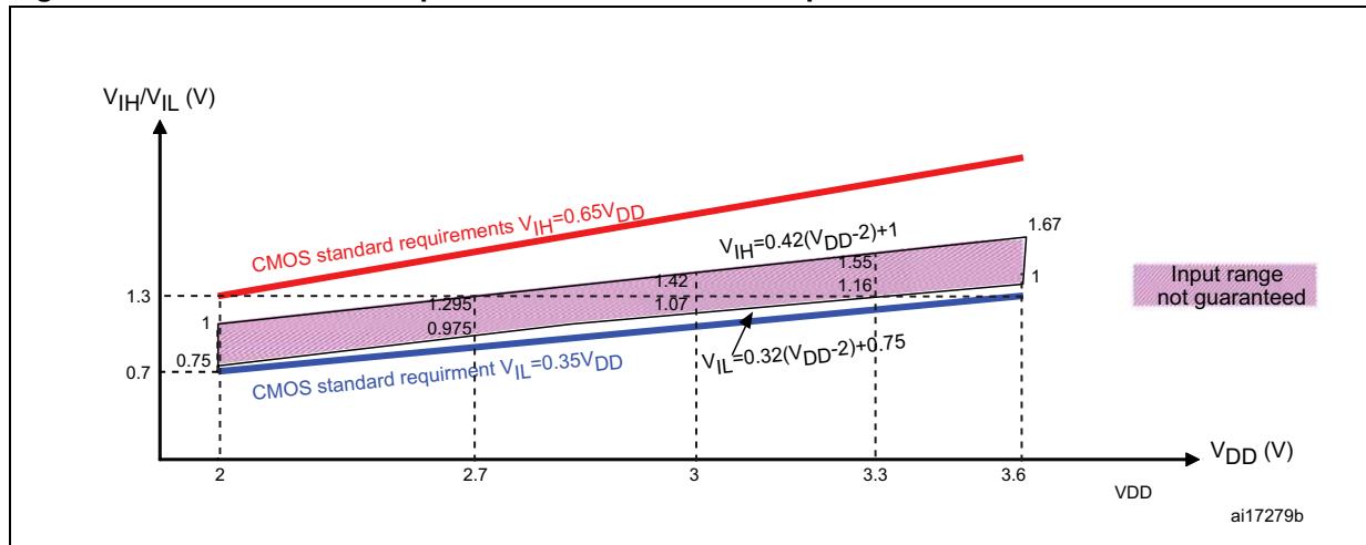
Figure 22. 5 V tolerant I/O input characteristics - CMOS port
