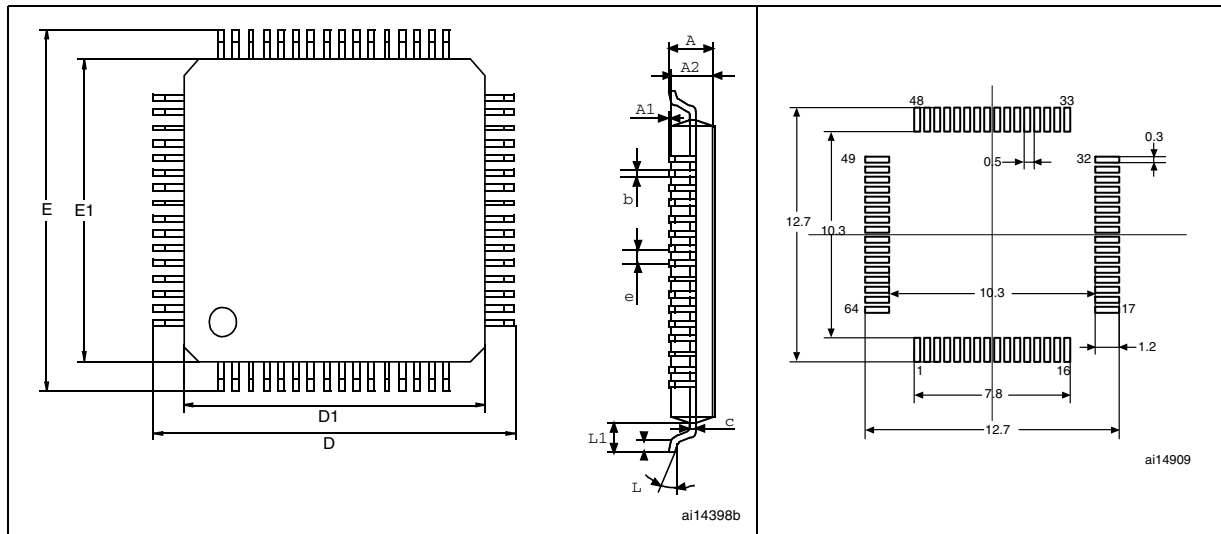
Figure 36. LQFP64 – 10 x 10 mm, 64 pin low-profile quad flat package outline (1) Figure 37. Recommended footprint (1)(2)
