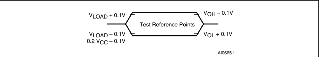
Figure 110. PSD Module AC float I/O waveform
