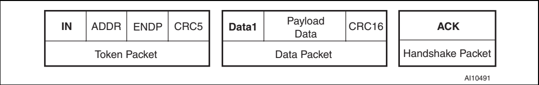
Figure 52. Interrupt Transfer
