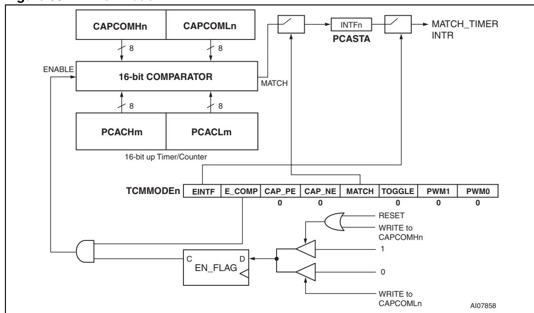
Figure 59. Timer mode
