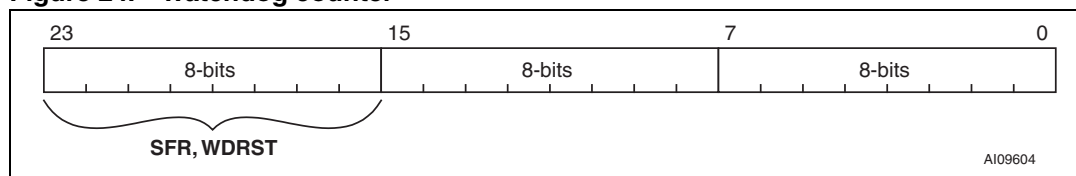
Figure 24. Watchdog counter
