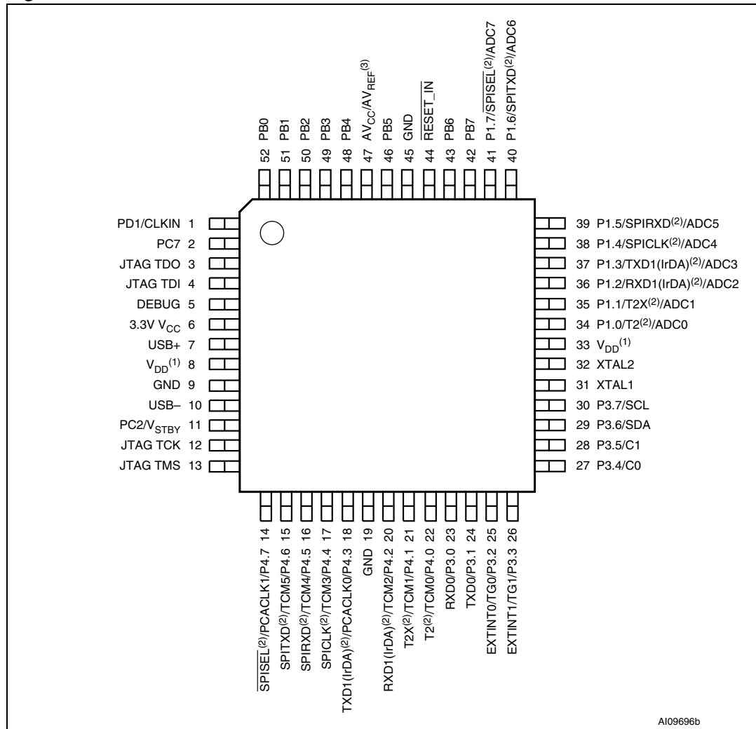
Figure 3. TQFP52 connections
