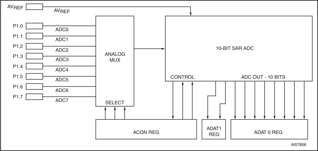
Figure 57. 10-bit ADC
