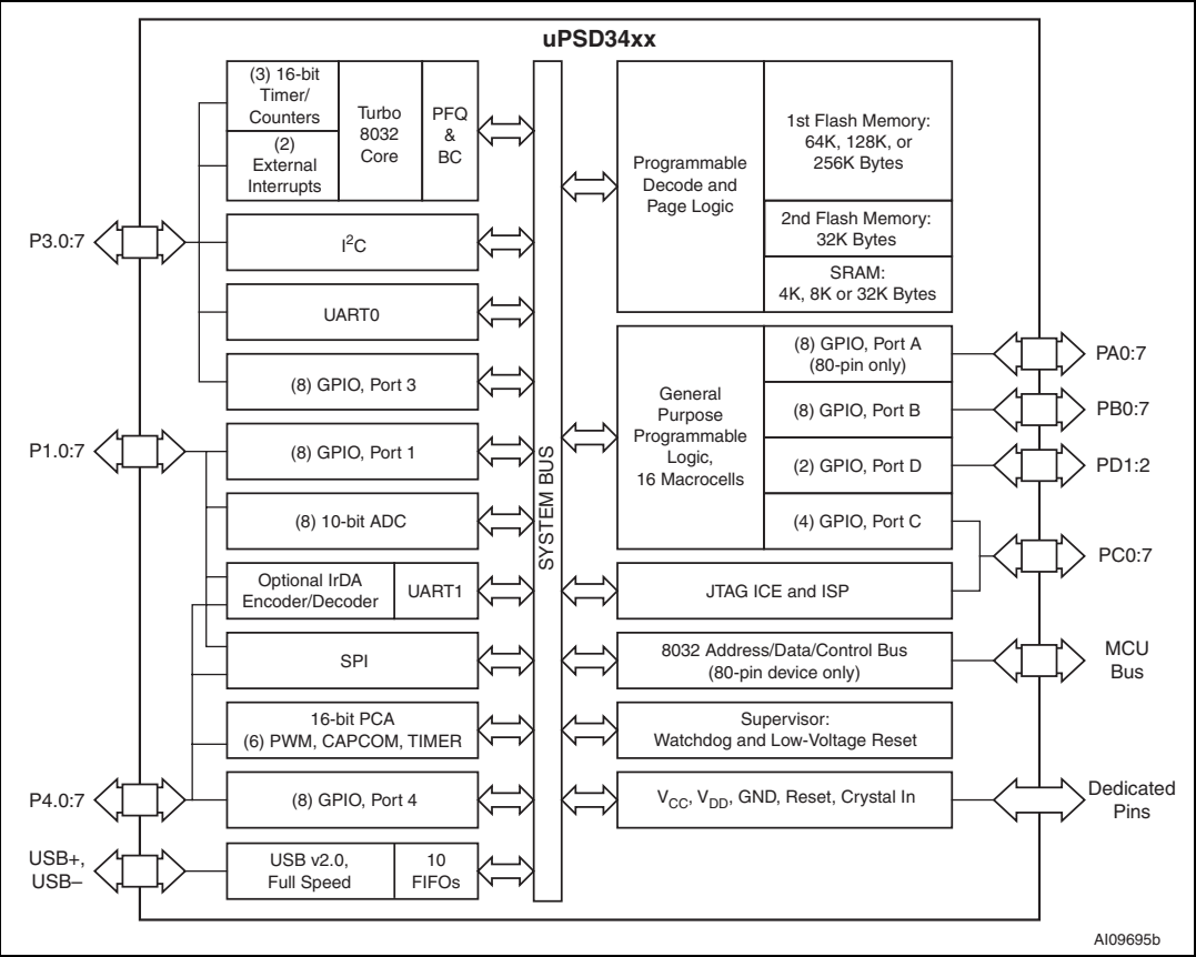
Figure 2. Block Diagram
