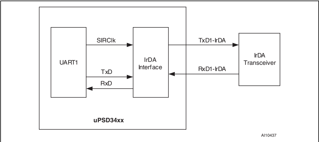
Figure 39. IrDA interface
