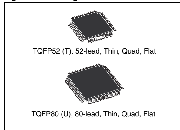
Figure 1. Packages
