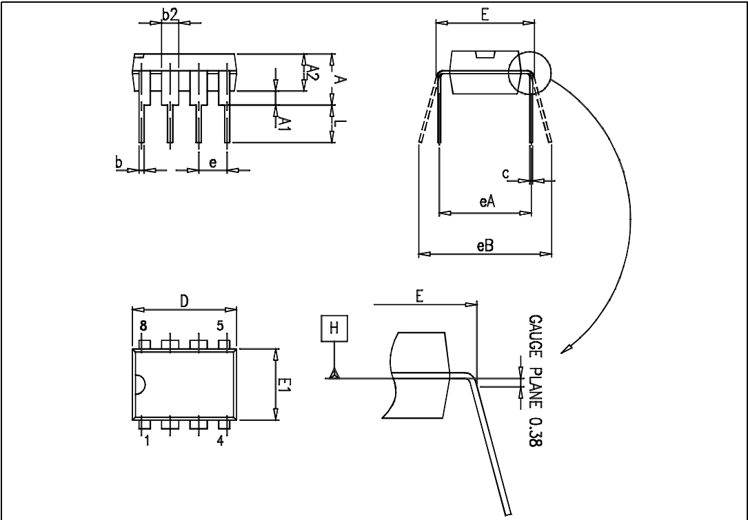
Figure 15. Package Dimensions
