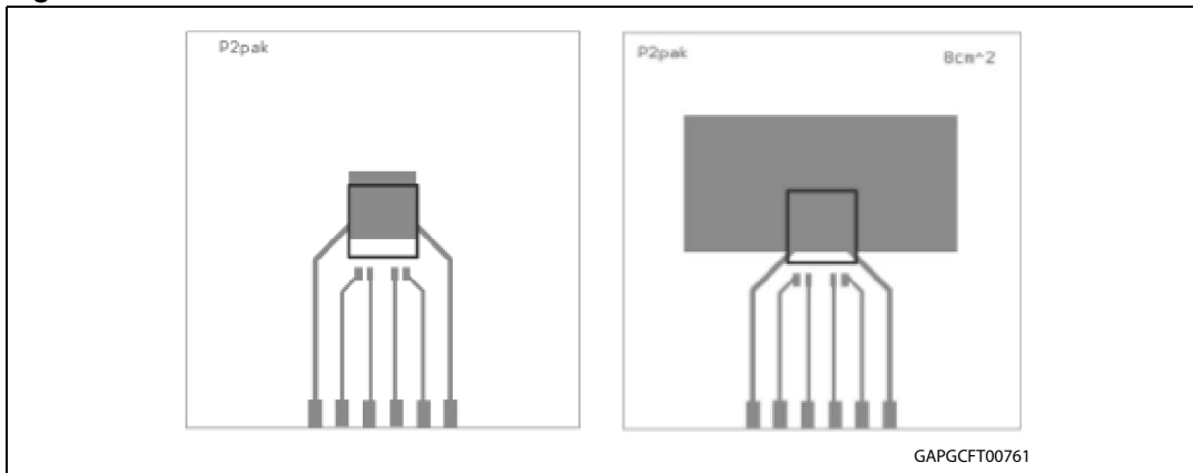
Figure 27. PC board
