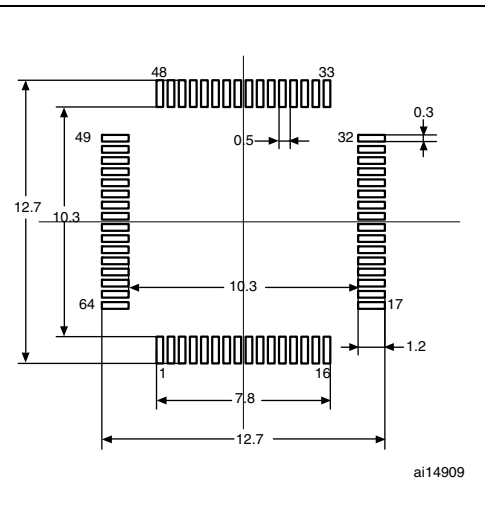
Figure 44. Recommended footprint (1)(2)
