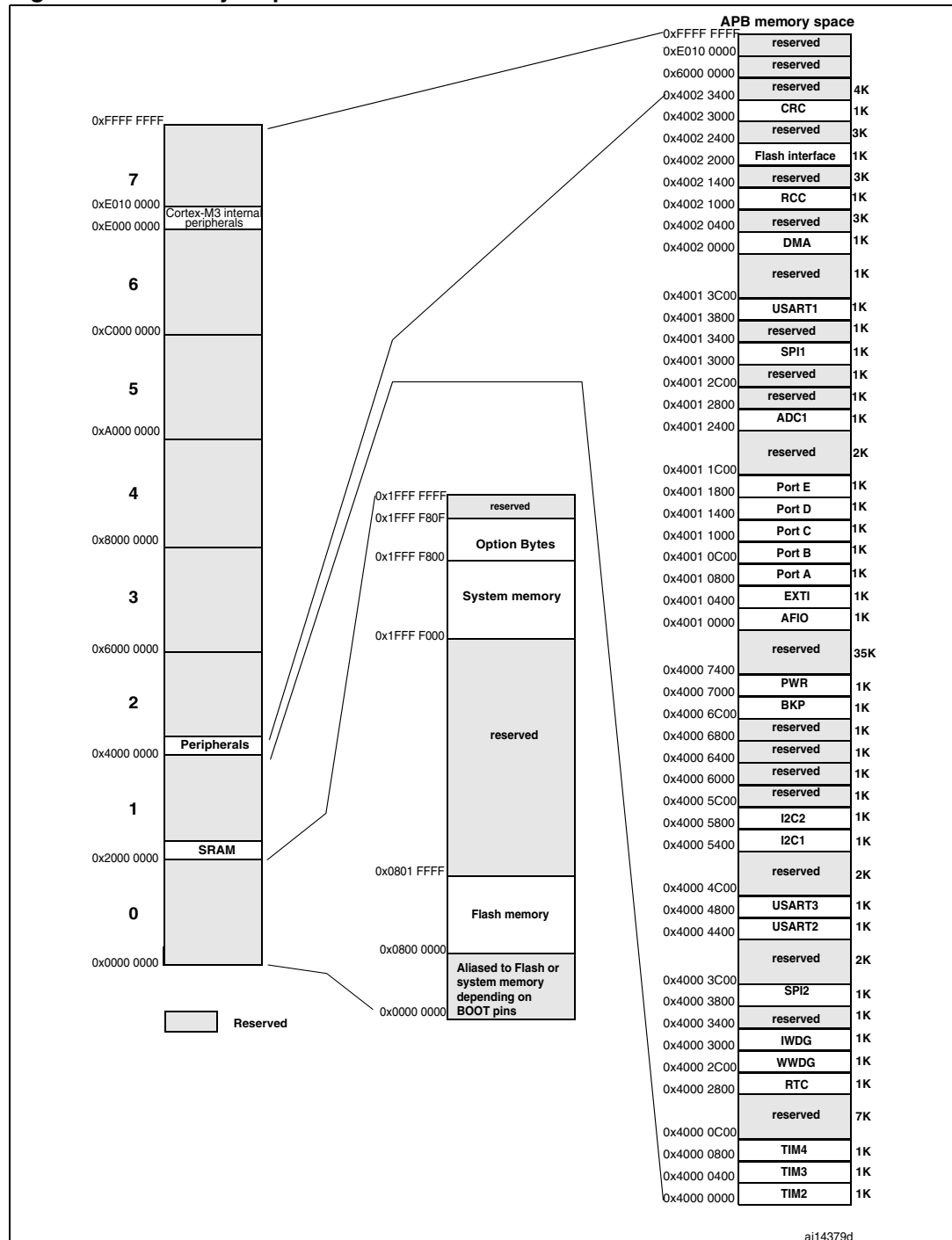
Figure 8. Memory map
