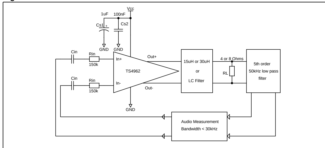
Figure 2. Schematic used for test measurements
