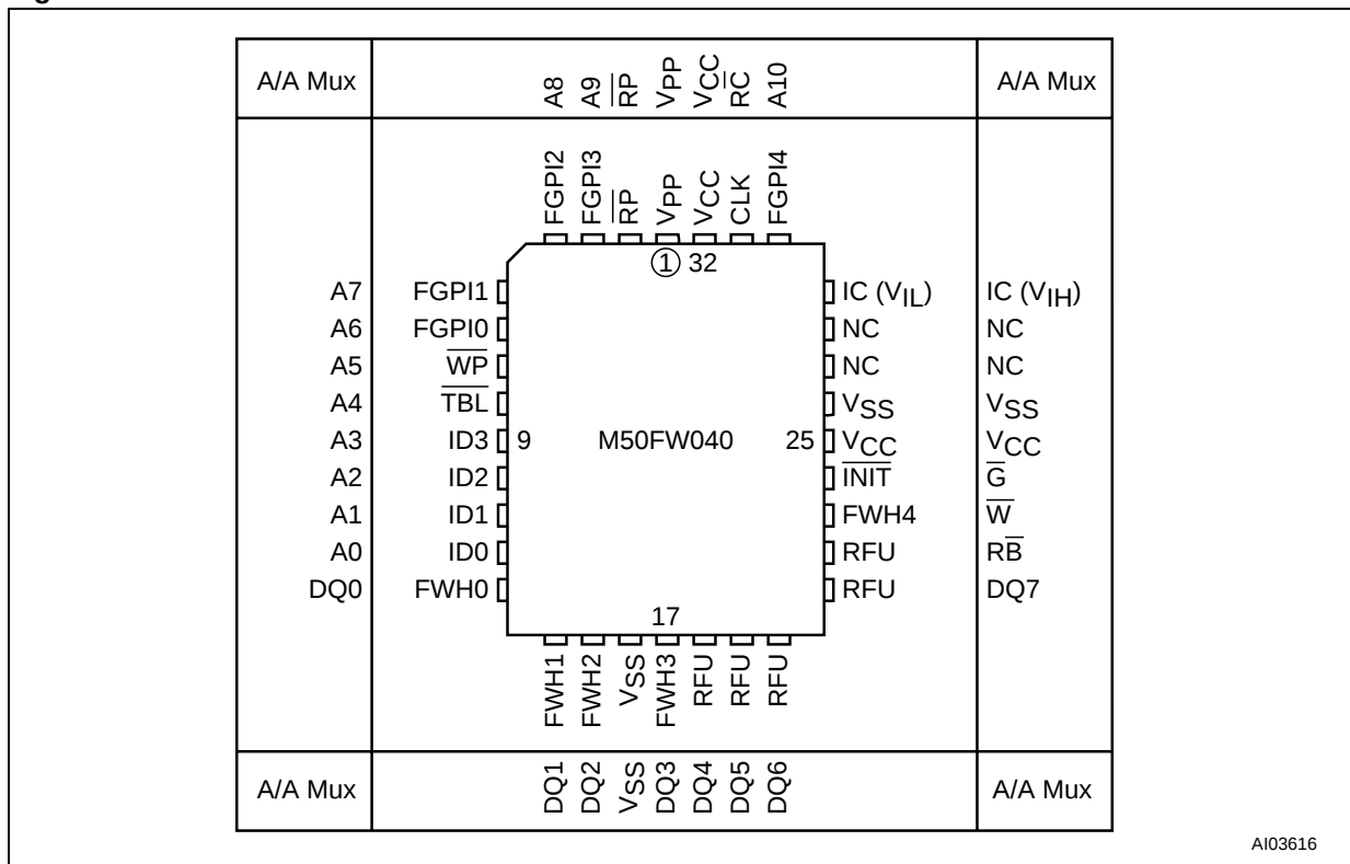
Figure 4. PLCC Connections
