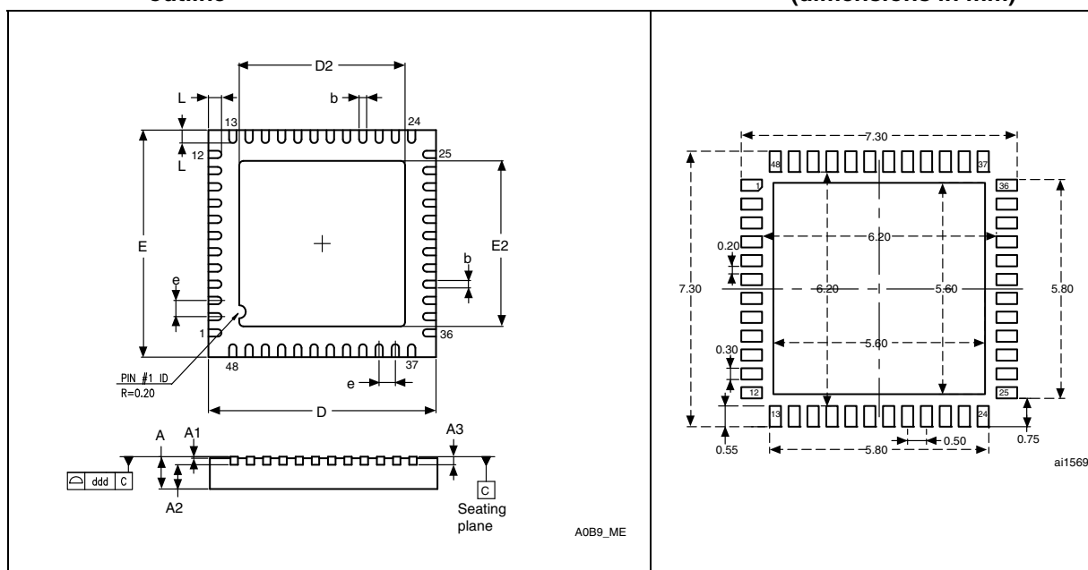
Figure 52. UFQFPN48 7 x 7 mm, 0.5 mm pitch, package outline (1)(2)(3)
