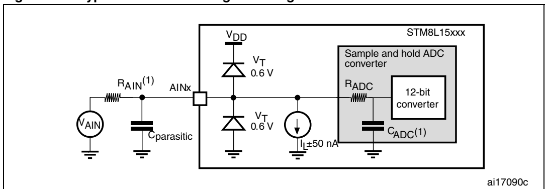
Figure 43. Typical connection diagram using the ADC
