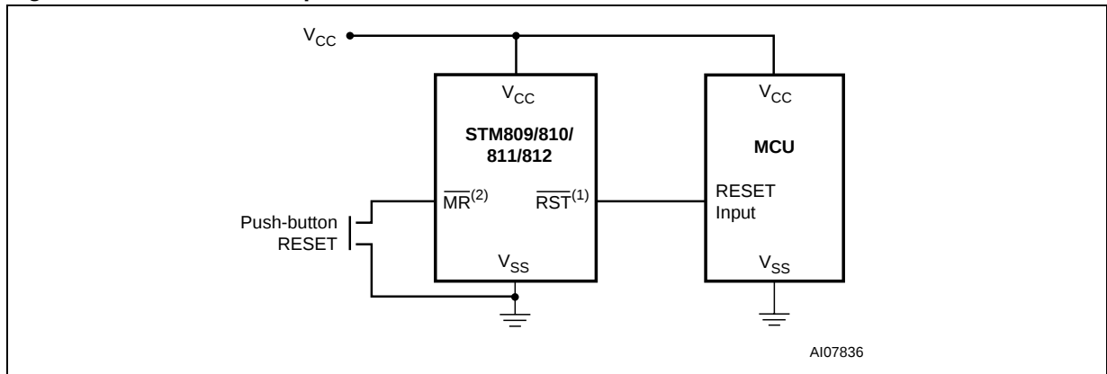
Figure 7. Hardware Hookup
