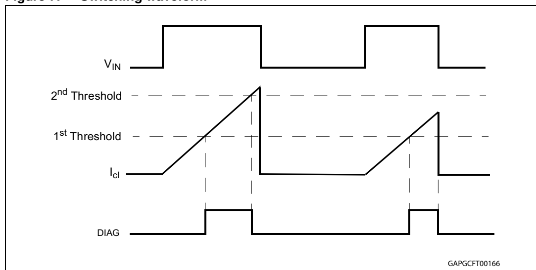
Figure 7. Switching waveform
