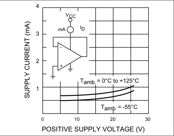
Figure 11. Supply current
