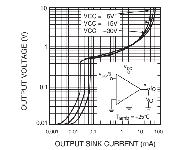
Figure 5. Current sinking output characteristics
