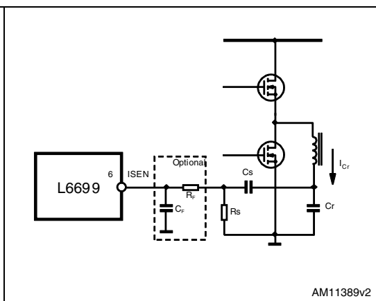
Figure 19. Current sensing techniques "lossless", with capacitive shunt
