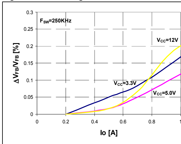
Figure 28. Load regulation
