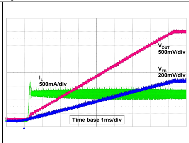
Figure 31. Soft start
