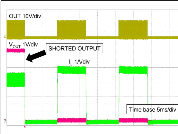
Figure 32. Short-circuit behavior
