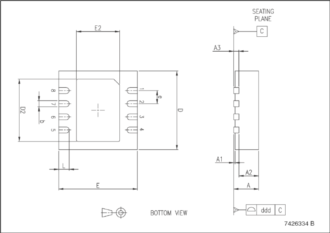
Figure 37. Package dimensions
