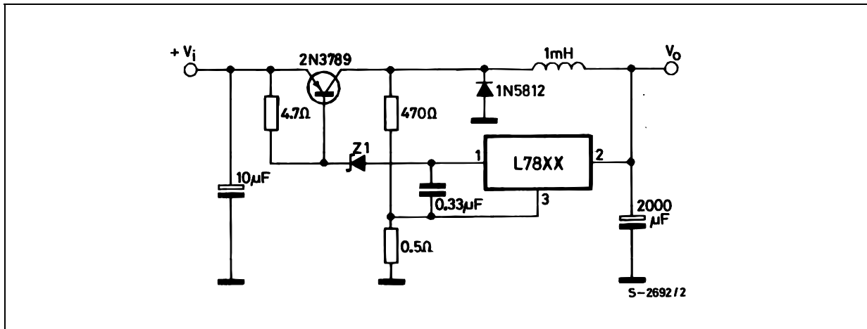
Figure 27. Switching regulator
