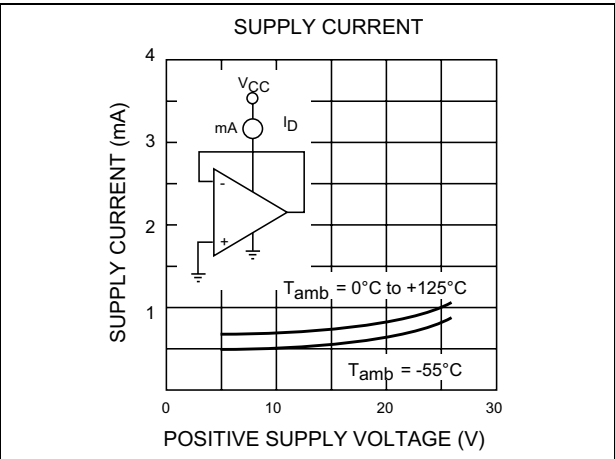
Figure 13. Supply current
