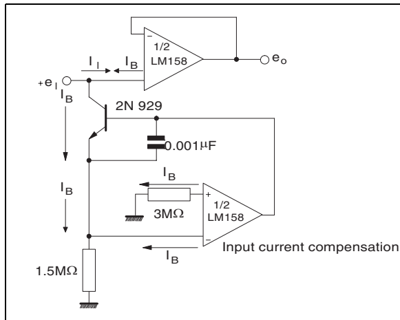
Figure 25. Using symmetrical amplifiers to reduce input current
