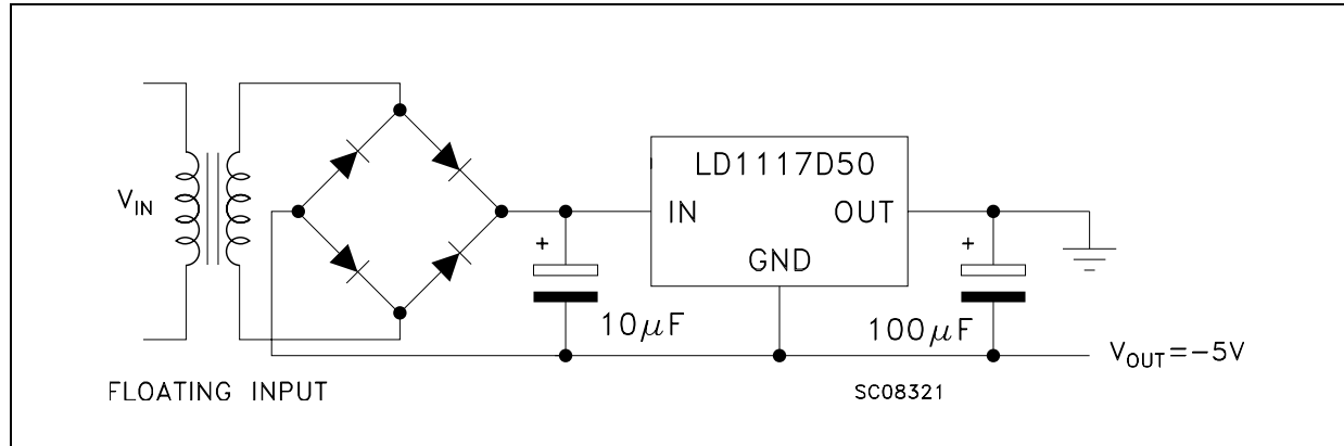
Figure 3. Negative supply
