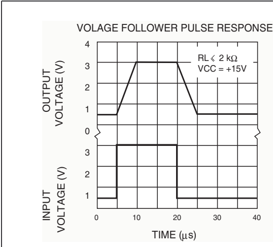
Figure 4. Voltage follower pulse response
