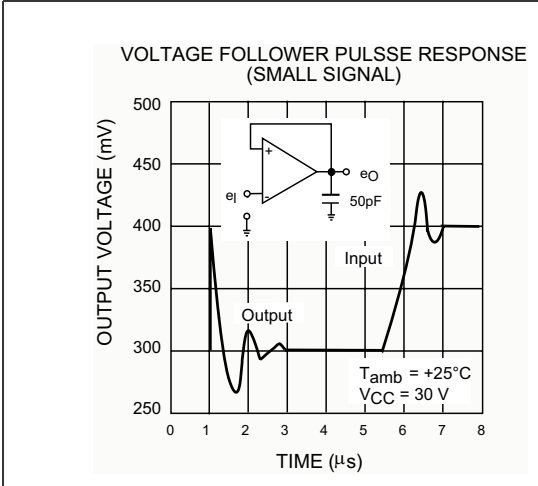
Figure 6. Voltage follower pulse response
