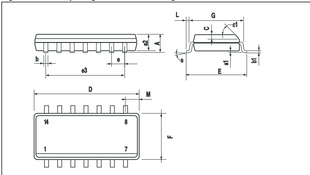
Figure 11. SO-14 package mechanical drawing
