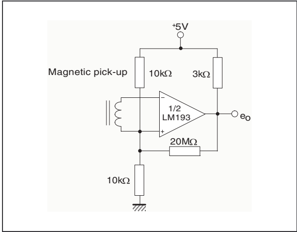
Figure 11. Transducer amplifier
