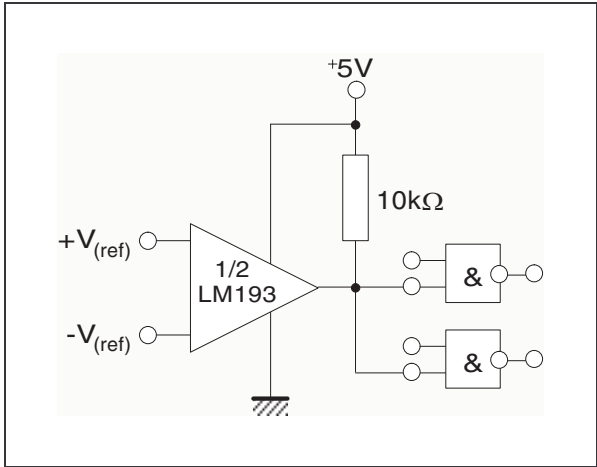
Figure 9. Driving CMOS
