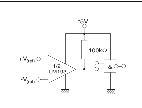
Figure 10. Driving CMOS
