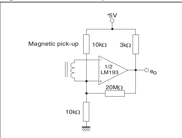
Figure 12. Transducer amplifier
