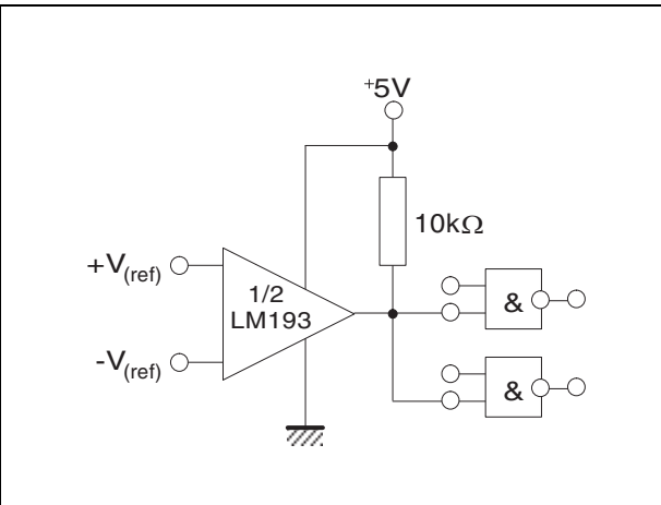
Figure 8. Driving TTL
