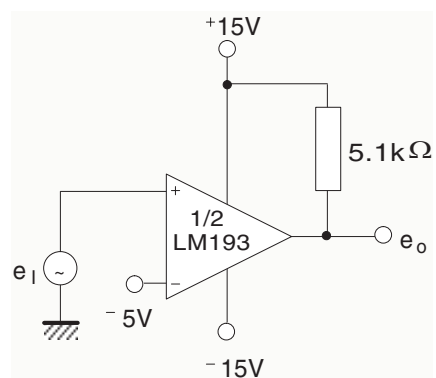
Figure 17. Comparator with a negative reference
