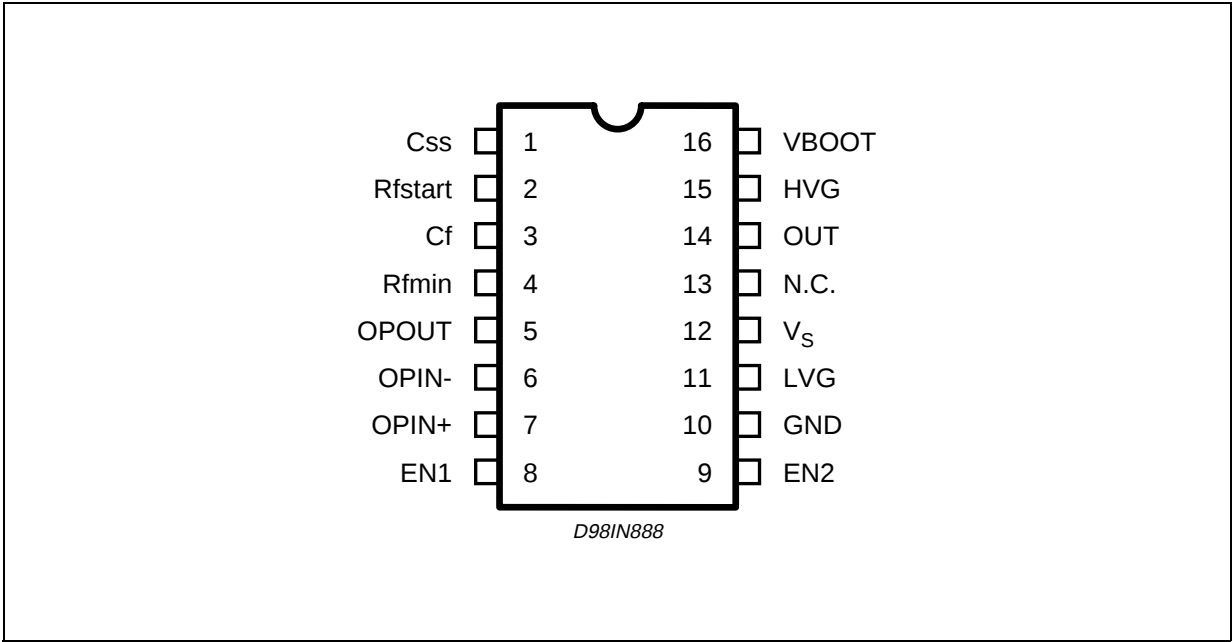
Figure 3. Pin Connection
