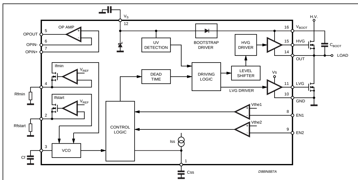
Figure 2. Block Diagram
