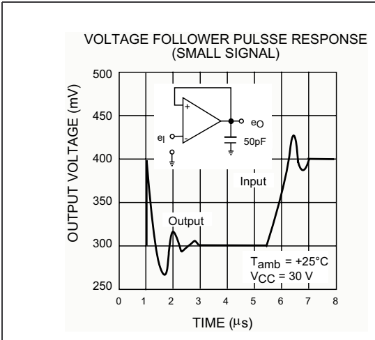
Figure 6. Voltage follower pulse response
