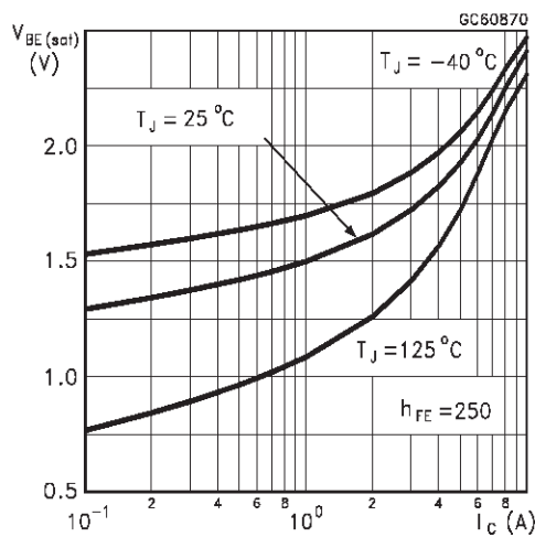
Base-Emitter Saturation Voltage (NPN type)
