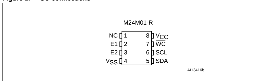
Figure 2. SO connections
