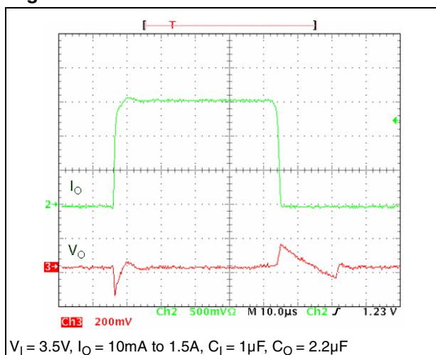
Figure 17. Load transient
