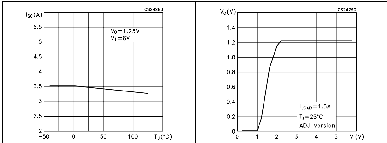
Figure 13. Short circuit current vs temperature Figure 14. Output voltage vs input voltage
