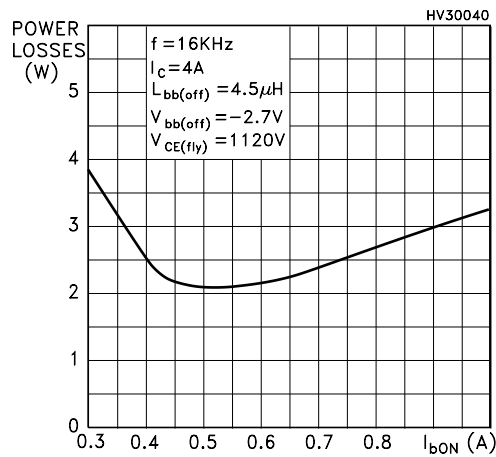
Figure 9. Power losses
