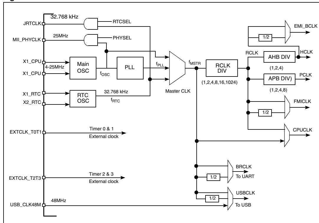
Figure 2. Clock control
