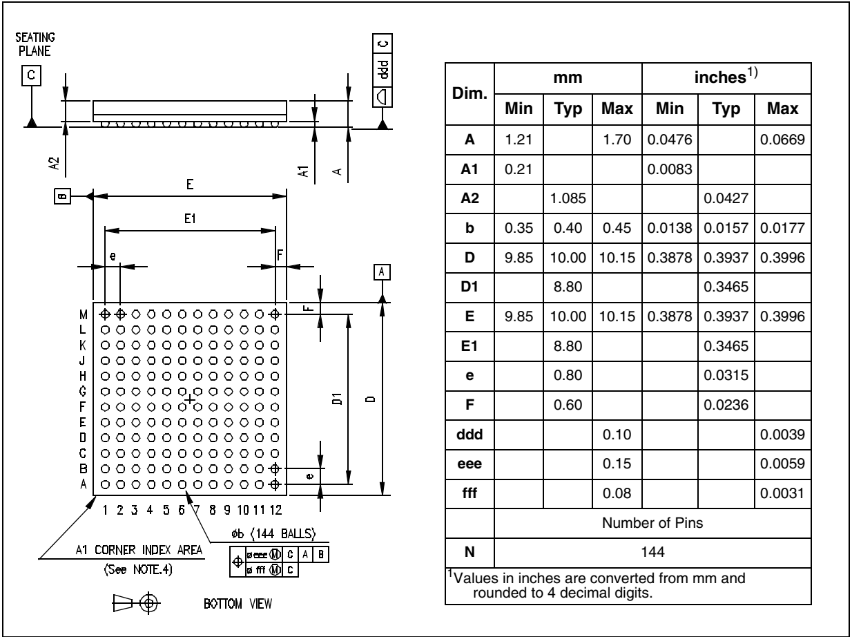
Figure 39. 144-ball low profile fine pitch ball grid array package (LFBGA144)
