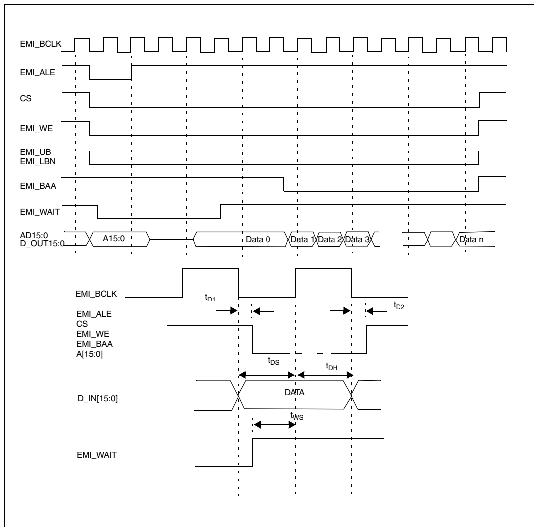
Figure 22. Sync burst write diagram
