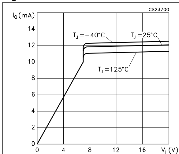
Figure 11. Quiescent current
