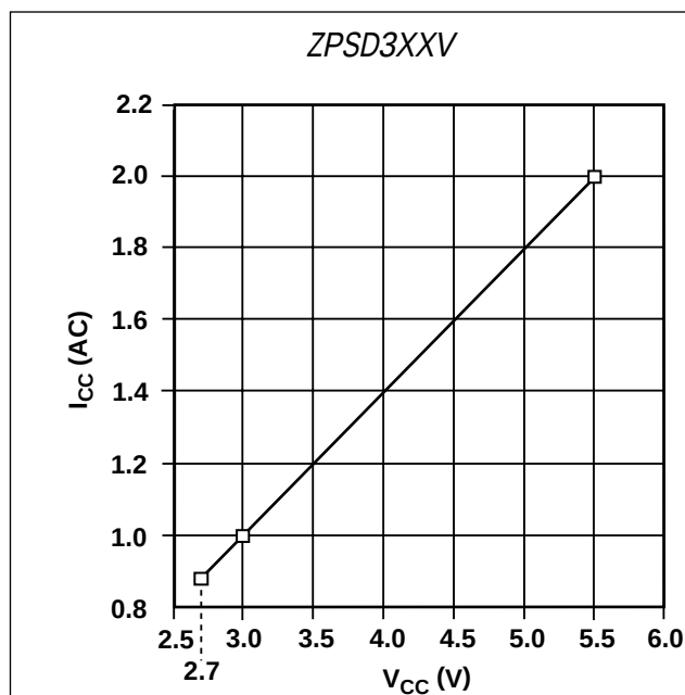
Figure 18. Normalized I_{CC} (AC) ( V_{CC} = 3.0\text{ V} )
