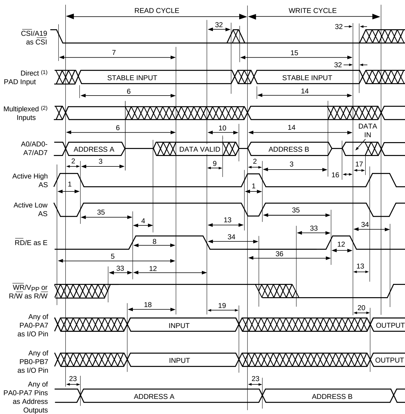
Figure 22. Timing of 8-Bit Multiplexed Address/Data Bus Using \overline{R}/\overline{W} , E or \overline{R}/\overline{W} , \overline{DS} (PSD3X1)
