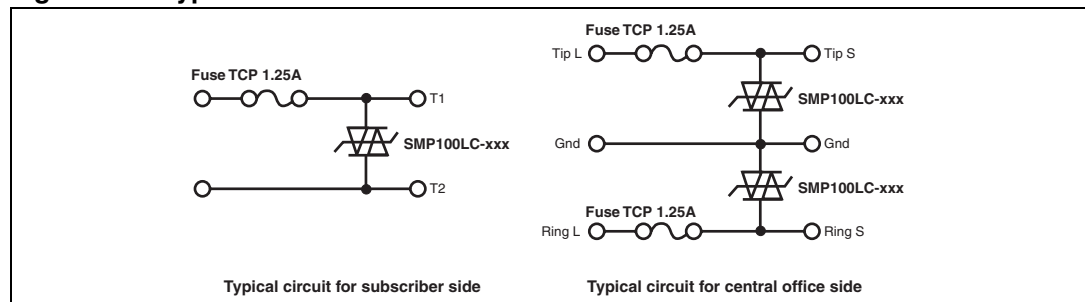
Figure 10. Typical circuits
