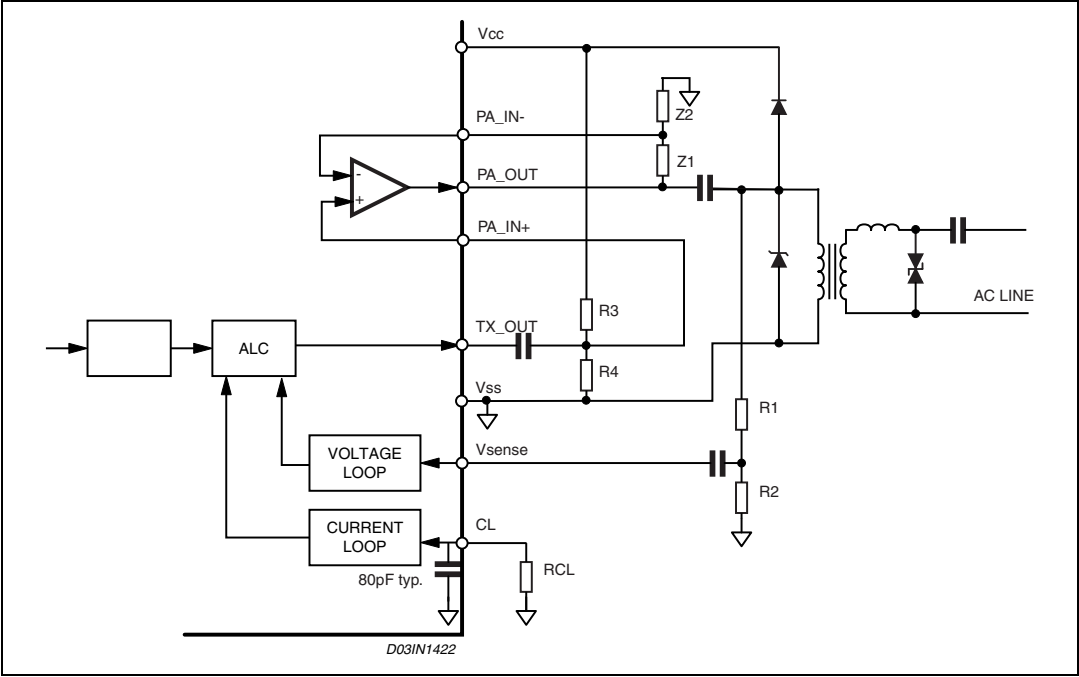
Figure 20. Power line interface topology
