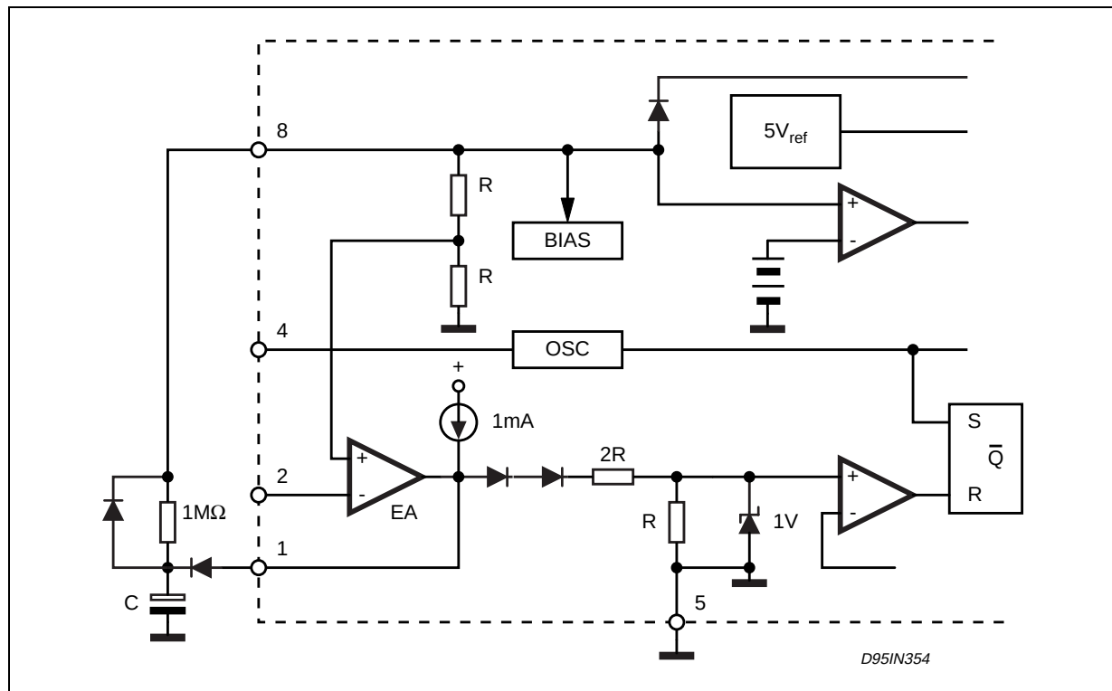
Figure 26. Soft-Start Circuit
