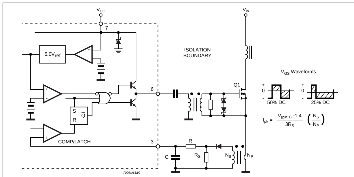
Figure 22. Latched Shutdown.
