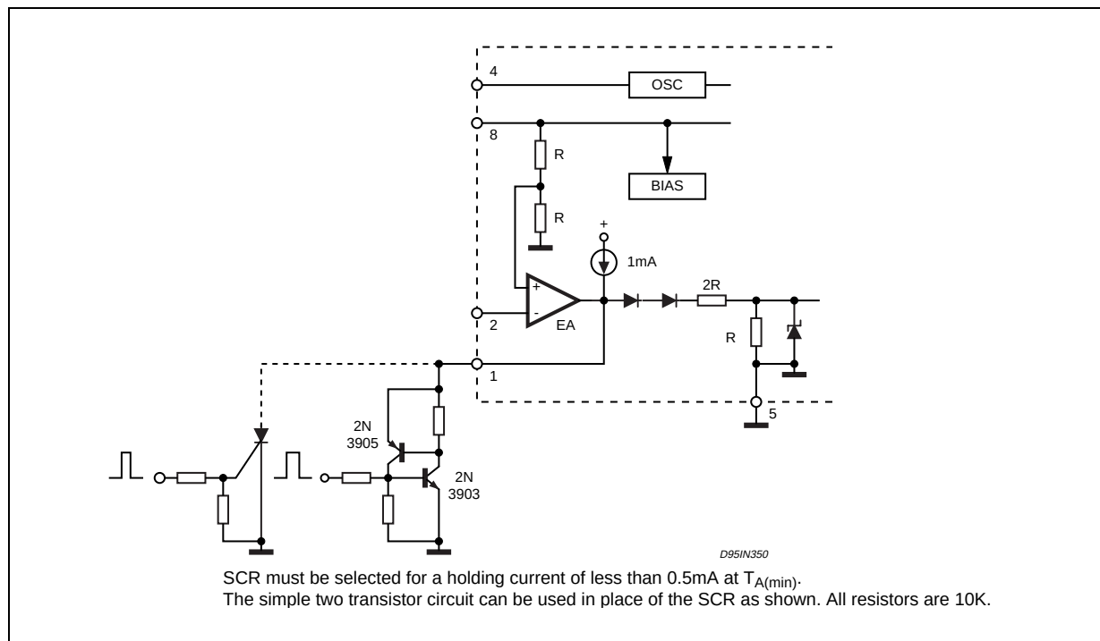
Figure 22. Latched Shutdown.
