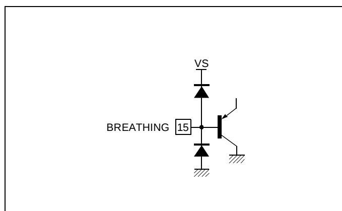
Figure 24: Breathing Input
