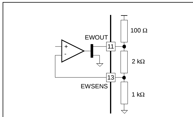
Figure 7: E/W Output
