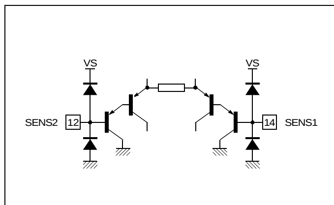
Figure 22: Vertical Current Sense
