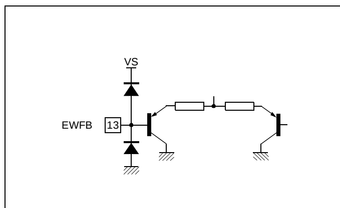
Figure 23: E/W Feedback
