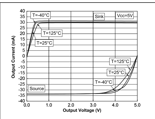
Figure 6. Output current vs. output voltage at V_{CC}=5\text{V}
