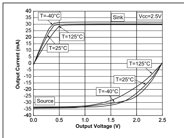
Figure 5. Output current vs. output voltage at V_{CC}=2.5\text{V}
