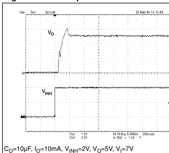
Figure 21. Start-up time 10 mA
