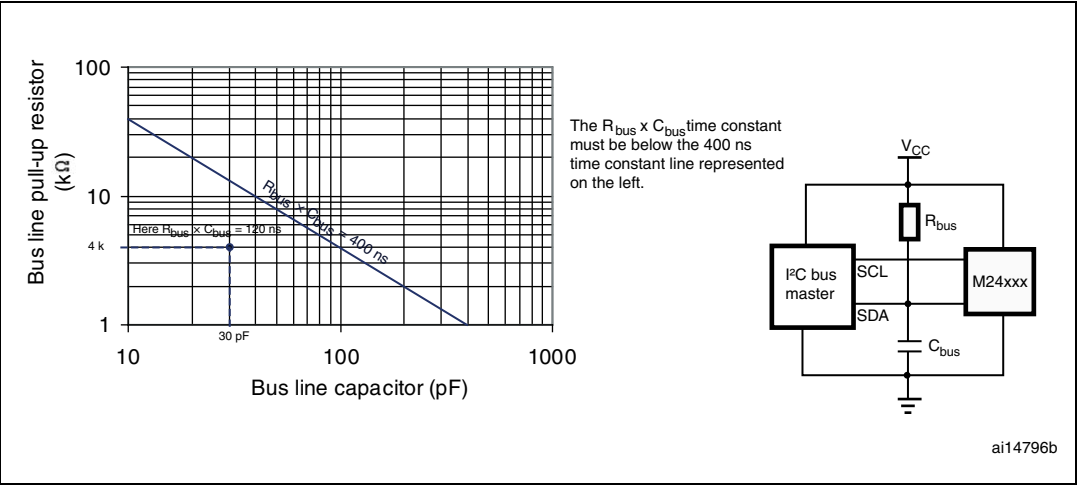
Figure 12. Maximum R_{bus} value versus bus parasitic capacitance ( C_{bus} ) for an I 2 C bus at maximum frequency f_C = 400\text{ kHz}
